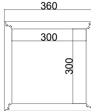
VISTA SUPERIOR S/ TAMPA
